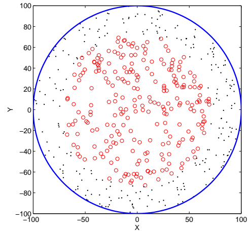
Fig. 10. Sensors that remain alive in the RS scheme after 50% of the sensor nodes run out of energy. Small circles represent alive sensor nodes, small dots represent dead sensor nodes.
