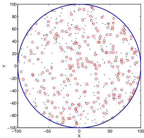
Fig. 12. Sensors that remain alive in the BS scheme after 50% of the sensor nodes run out of energy. Small circles represent alive sensor nodes, small dots represent dead sensor nodes.
