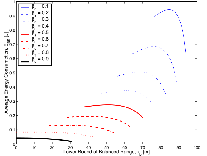
Fig. 2. Energy Consumption of the BS Scheme for Different \beta_s ( \gamma = 2 ).
