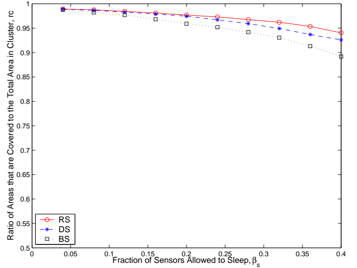
Fig. 6. Comparison of sensing coverage of RS, DS, and BS schemes ( \gamma = 2 ).
