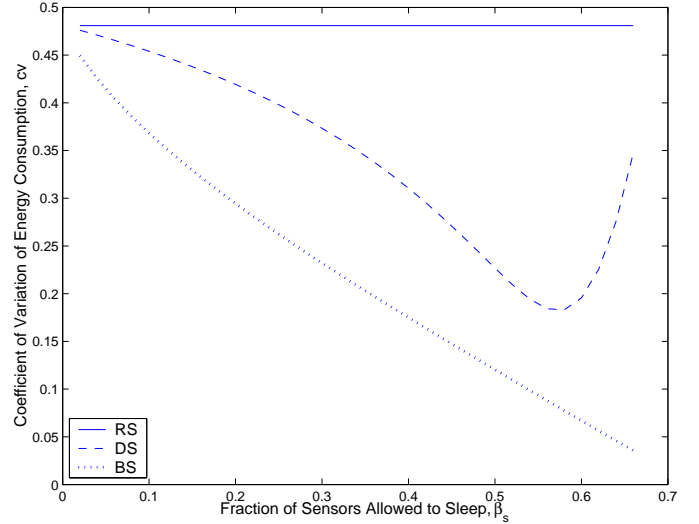
Fig. 4. Coefficient of Variation Comparison of the RS, DS, and BS schemes ( \gamma = 2 ).
