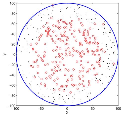
Fig. 11. Sensors that remain alive in the DS scheme after 50% of the sensor nodes run out of energy. Small circles represent alive sensor nodes, small dots represent dead sensor nodes.
