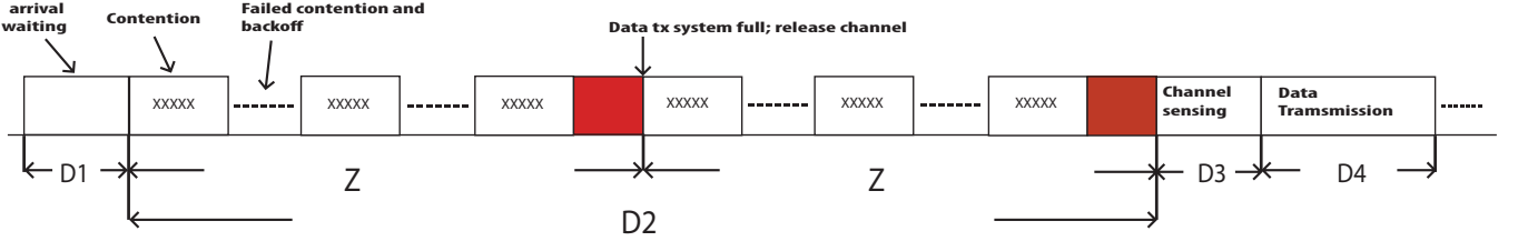
Fig. 2. O-MAC scheme: “cs” denotes channel sensing
