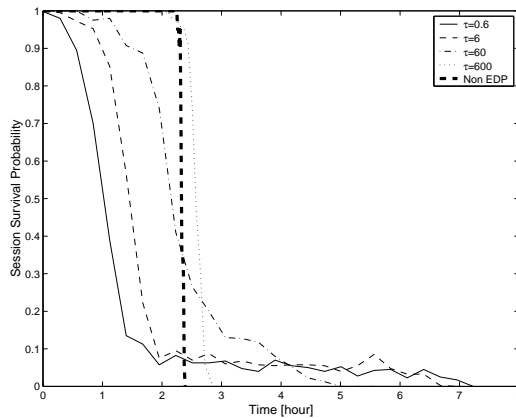
Fig. 5. Session survival probability, without partition checking
