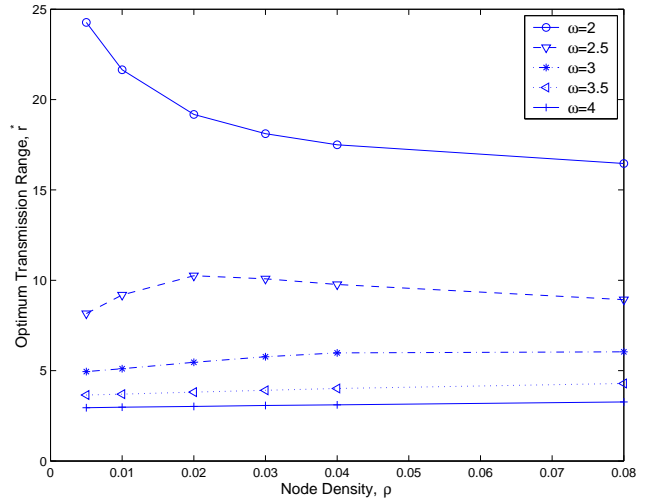
Fig. 8. Optimum transmission range for different \omega .
