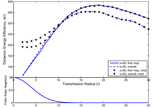
Fig. 12. Distance-energy efficiency for \rho = 0.02 and \omega = 2 . The sub-figure below depicts the probability of no relay neighbor in the range of transmission radius. This probability is calculated as E_V[P_0(v, r)] = \int_r^x e^{-\rho A_{SD}(v, r)} (2v/x^2) dv [18]. The optimal transmission radii respectively for first-hop, first-hop (mod), overall, overall (mod) are 16, 16, 18, and 18, which result in the energy-efficiencies of 381, 376, 353, and 352, respectively.
