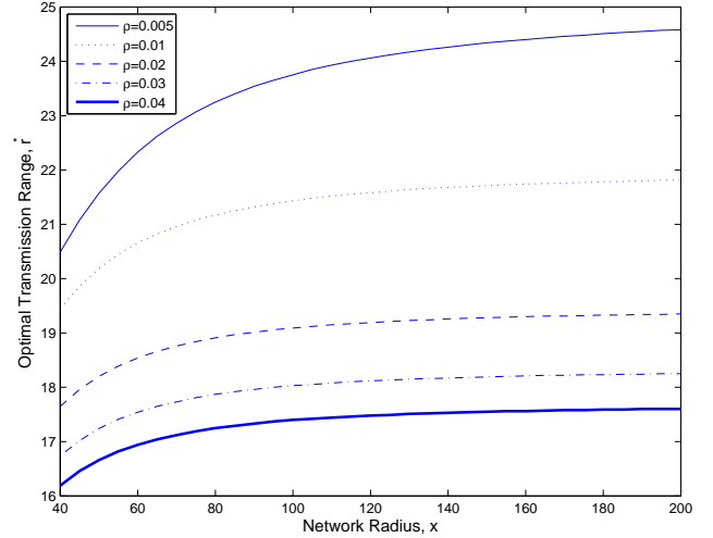
Fig. 7. Optimum transmission range for different node densities ( \omega = 2 ).
