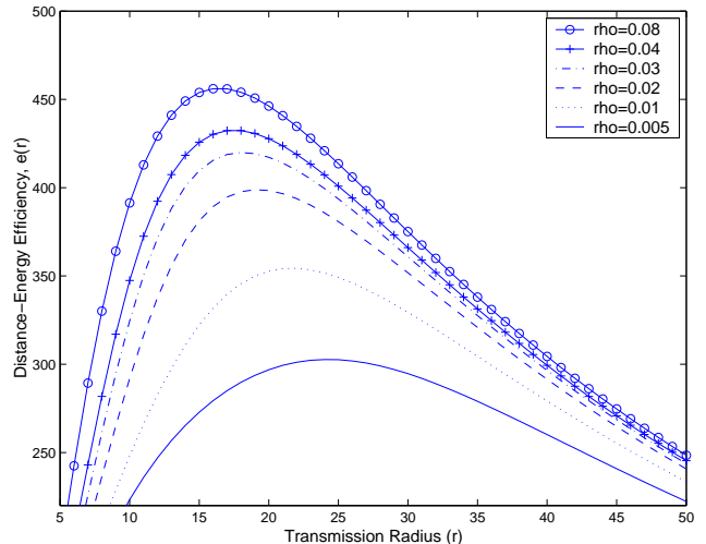
Fig. 4. Distance-energy efficiency ( \omega = 2 ).
