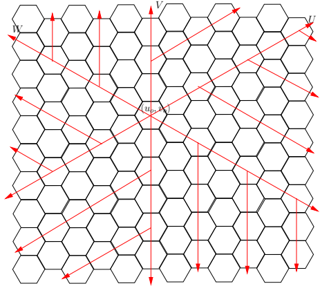
Fig. 4. The GB(n = 3) Scheme, \Phi_r \geq 1 - (1 - p_r)^3
